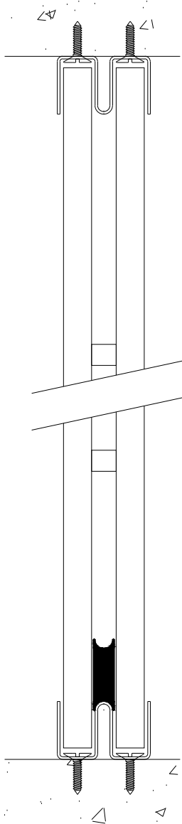
BOTTOM ROLLING REVEAL FIX
