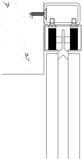
TOP HUNG FACE FIX
